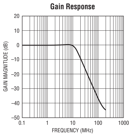
660510 F05a \pm 0.7\text{dB} 11.2MHz PASSBAND GAIN = 1\text{V/V} (0dB) Z_{\text{IN}} = 800\Omega
